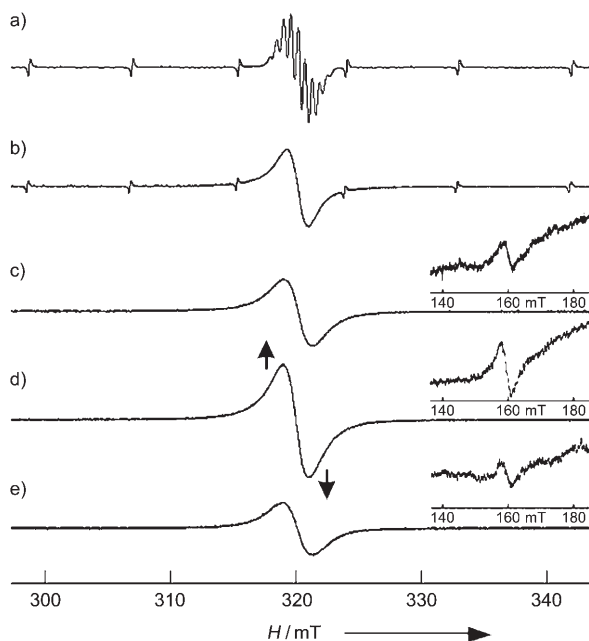
Figure 2. ESR spectra of a) ligand 1 (295 K, \text{CHCl}_3/\text{MeOH}=4:1 , 4 mM, g=2.003 ); b) cage 2 (293 K, \text{H}_2\text{O} , 1 mM, g=2.003 ); c) cage 2 (113 K, frozen \text{H}_2\text{O} , 1 mM, g=2.003 ); d) complex 2·3 (113 K, frozen \text{H}_2\text{O} , 1 mM, g=2.004 ); e) recovered 2 after extraction of 3 with \text{CHCl}_3 from 2·3 (113 K, frozen \text{H}_2\text{O} , 1 mM, g=2.003 ). The intensity is normalized. The insets show the forbidden transition ( \Delta m_s=2 ) which was measured using 16 mW microwave power.
