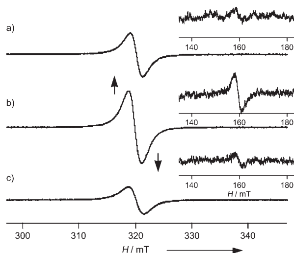
Figure 3. ESR spectra of a) cage 2 (113 K, frozen \text{H}_2\text{O} , 1 mM, g=2.003 ); b) complex 2·(4) 2 (113 K, frozen \text{H}_2\text{O} , 1 mM, g=2.004 ); c) recovered 2 after extraction of 4 with \text{CHCl}_3 from complex 2·(4) 2 (113 K, frozen \text{H}_2\text{O} , 1 mM, g=2.003 ). The intensity is normalized. The insets show the forbidden transition ( \Delta m_s=2 ), which was measured using 1 mW microwave power.
